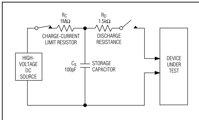
Figure 3a. Human Body ESD Test Model
